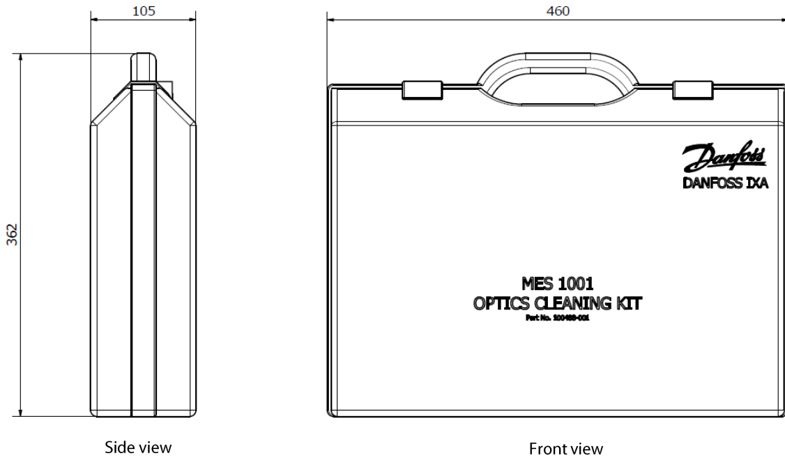
Illustration 1: Dimensions All dimensions are in mm.
